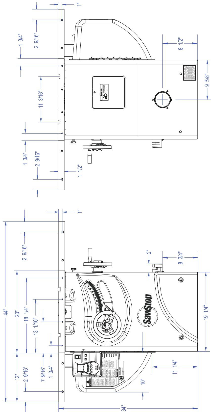
Front View
