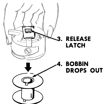
Fig. 10. Removing Bobbin from Bobbin Case
