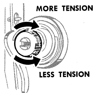
Fig. 21. Regulating Needle Thread Tension
