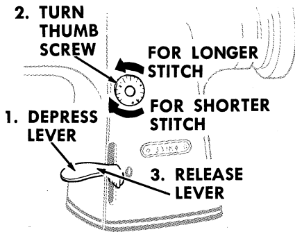
Fig. 24. Regulating Length of Stitch on Machine 331K4
