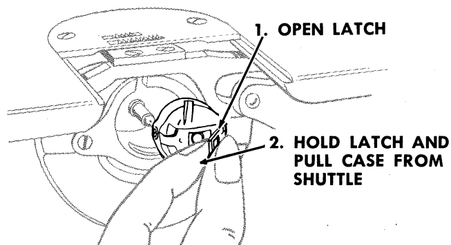
Fig. 9. Removing Bobbin Case and Bobbin from Machine
